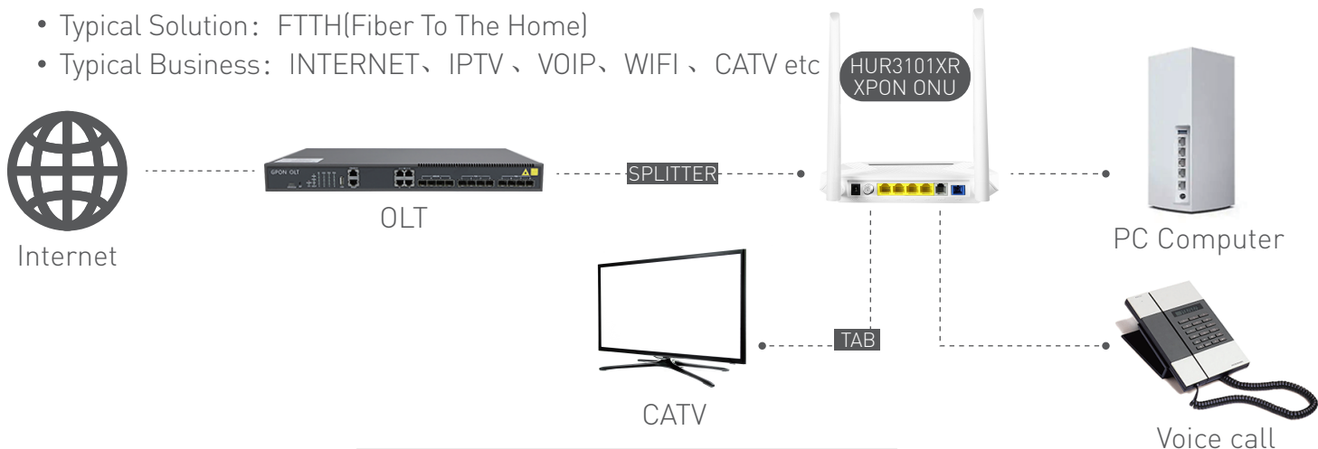
Figure: HUR3101XR Application Diagram
